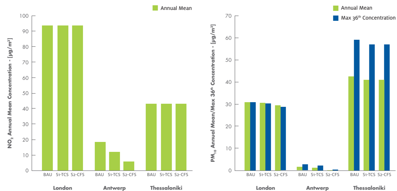
FIGURE 5. a) NO 2 AND b) PM 10 AIR QUALITY LEVELS AT THE RESPECTIVE MONITORING LOCATIONS UNDER THE THREE ANALYSED SCENARIOS
